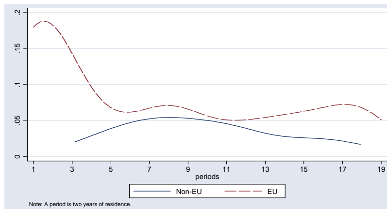
FIGURE 3: Smoothed Hazard Function by EU Status
