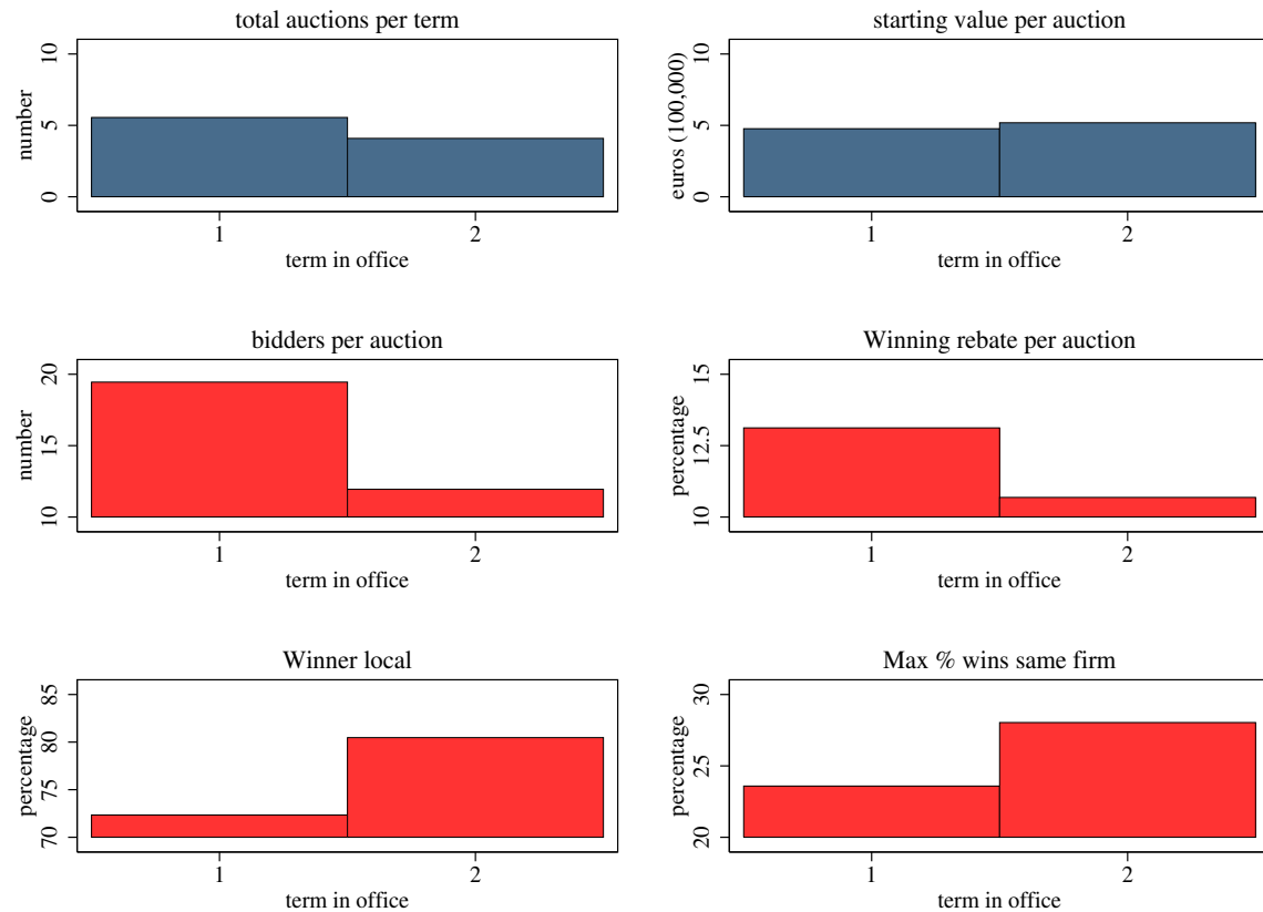
Figure 2: Auctions' characteristics across terms (no term limit in the second term)
