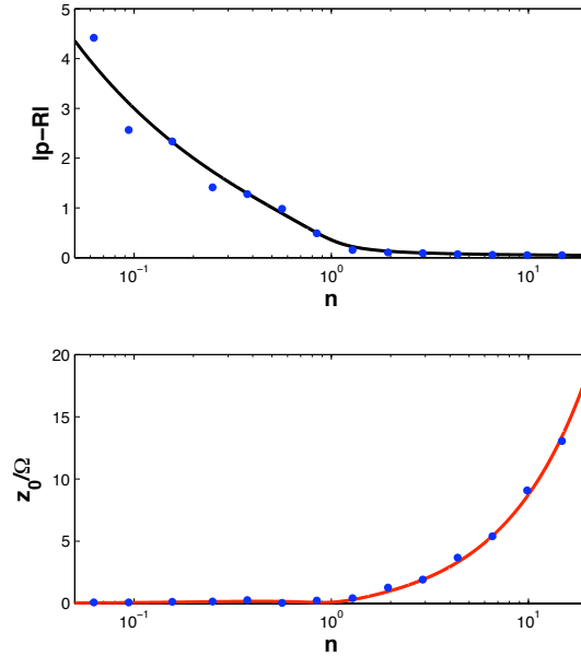
Figure 1: Top panel: distance |p - R| = \sqrt{\sum_{\omega=1}^{\Omega} E_{k_0} [R^{\omega} - p^{\omega, k_0}]^2} of prices from dividends in competitive equilibrium. The full line represents the analytical solution for the case s = \bar{R} = 1 and \varepsilon = 0.1 , points refer to numerical simulations of systems with \Omega = 32 , s = \bar{R} = 1 and \varepsilon = 0.1 . Bottom panel: monetary amount invested by the trend follower z_0 for the same values of the parameters.
