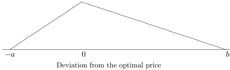
Figure 1: The long-run density function.
