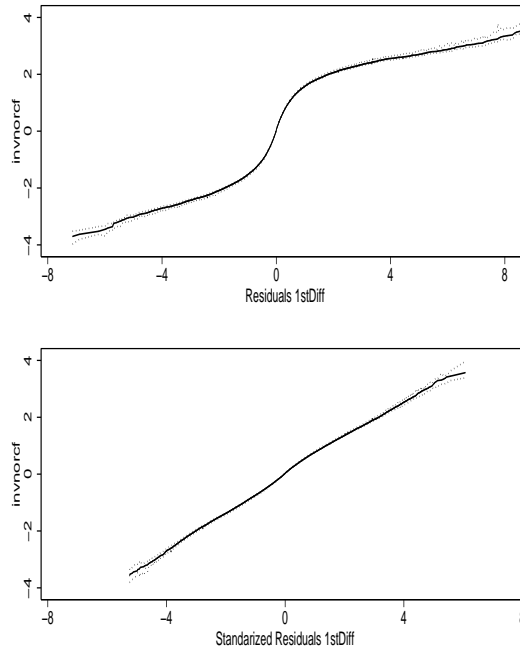
Figure 4. Distribution of Residuals and Standardized Residuals in First Differences.
