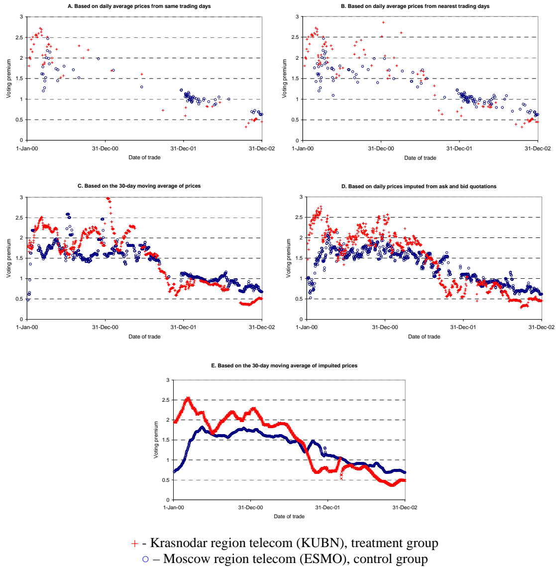
Figure 1. Different approaches to calculating the voting premium.
