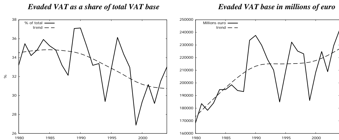
Figure 1: VAT undeclared tax base (solid line) and long-run trend (dashed line)
