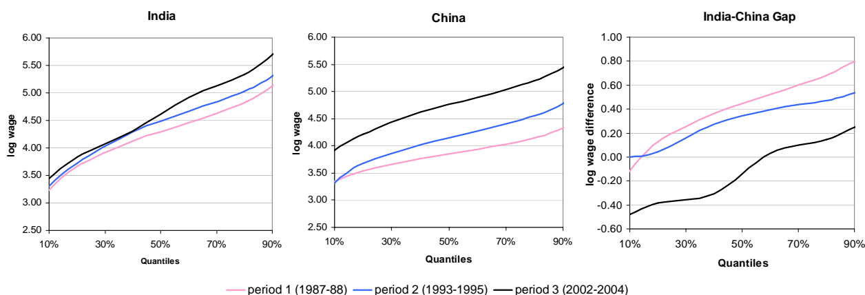
Figure 1: Log-wage Distributions
