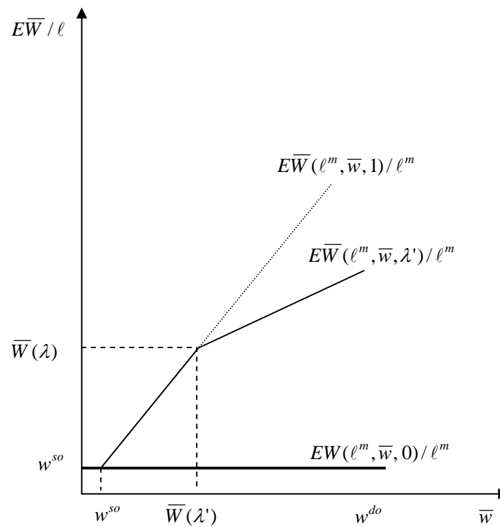
Figure 5 Expected Labor Cost per Worker
