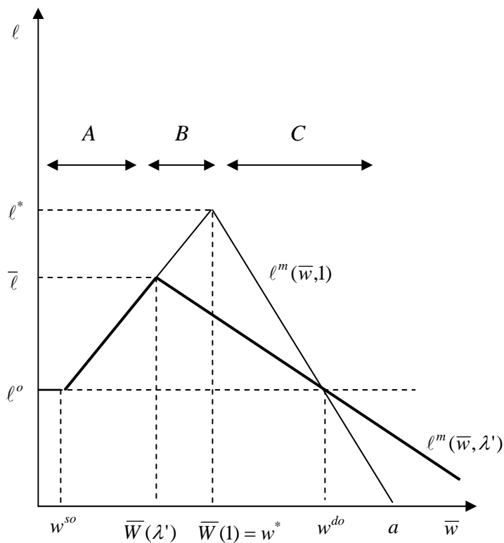
Figure 4 Employment and Minimum Wage With Imperfect Enforcement A: No Change B: Sign Reversal C: Muted Response
