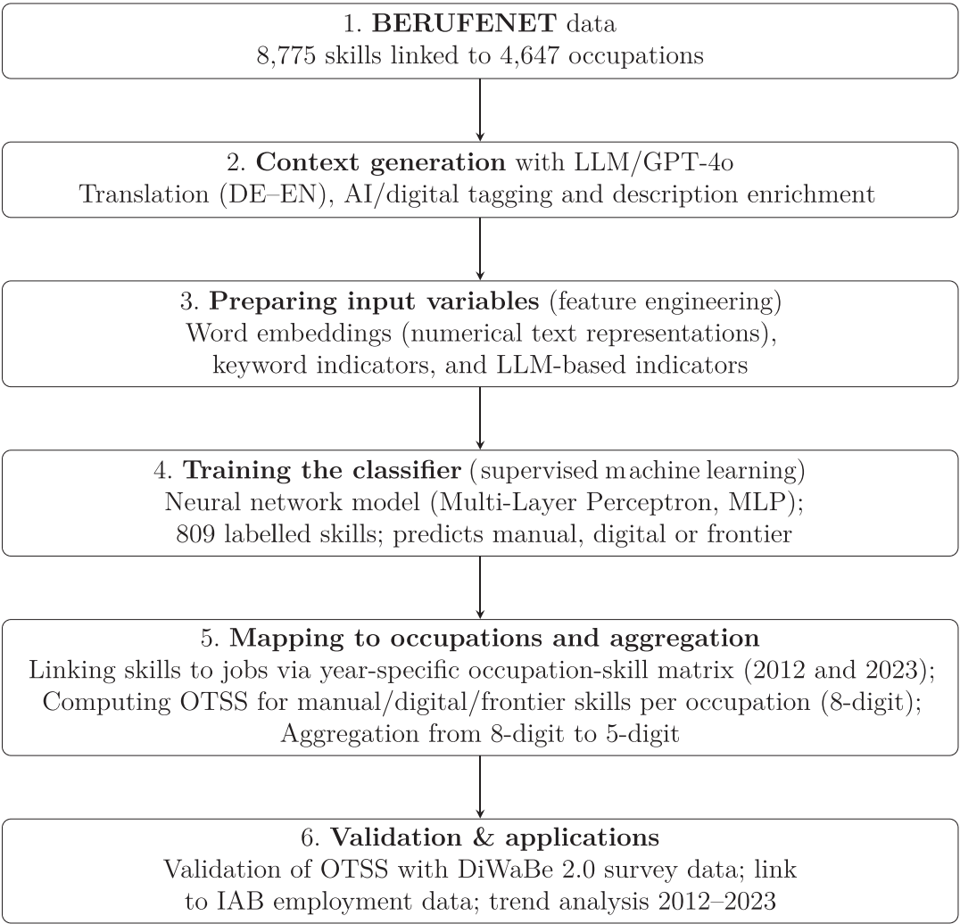
FIGURE 1 Overview of the AI-powered skill classification pipeline and OTSS construction. Note: The figure summarises the workflow from data collection and contextual enrichment to supervised machine-learning classification of skills, construction of OTSS and validation for 2012 and 2023.
