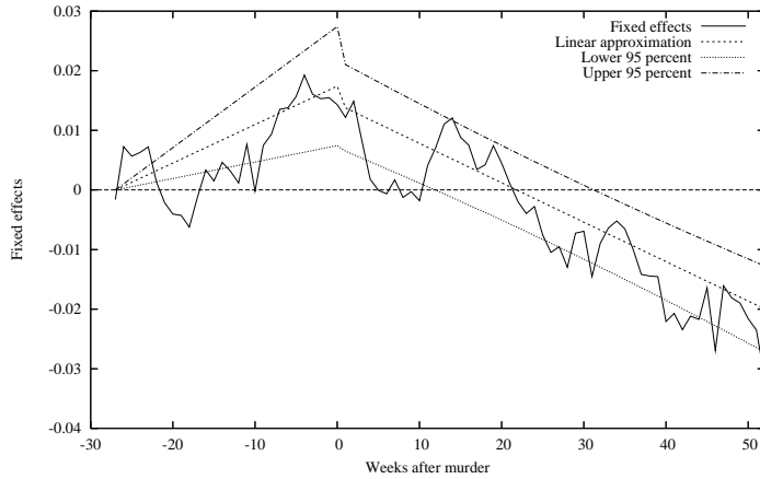
Figure 7: Quality of the approximation: the linear model.
