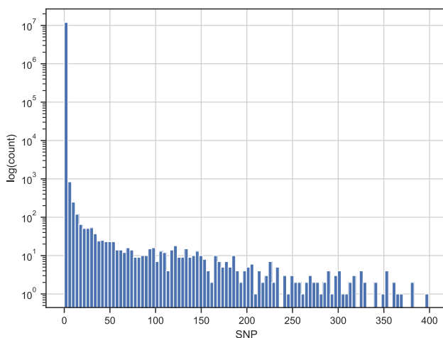
Fig. 3 Distribution of SNP for all users in dataset
