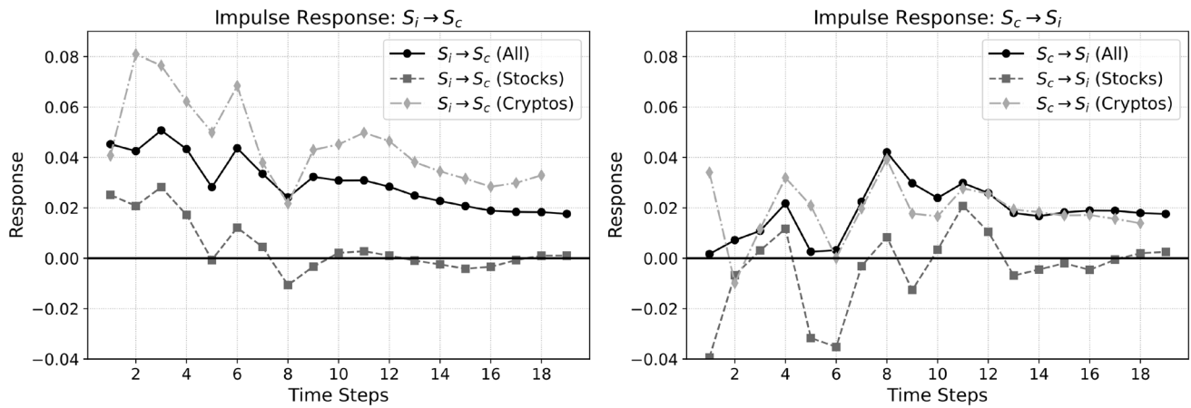
Fig. 4 Impulse response functions for S_i \rightarrow S_c and S_c \rightarrow S_i
