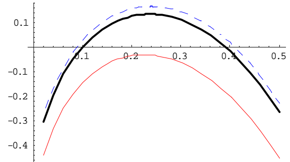
Figure 6b: Changing \delta
