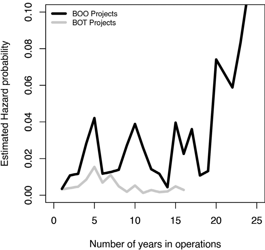
Fig. 4. Hazard Functions for BOT and BOO Projects.
