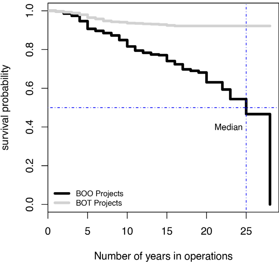
Fig. 5. Survival Functions for BOT and BOO Projects.
