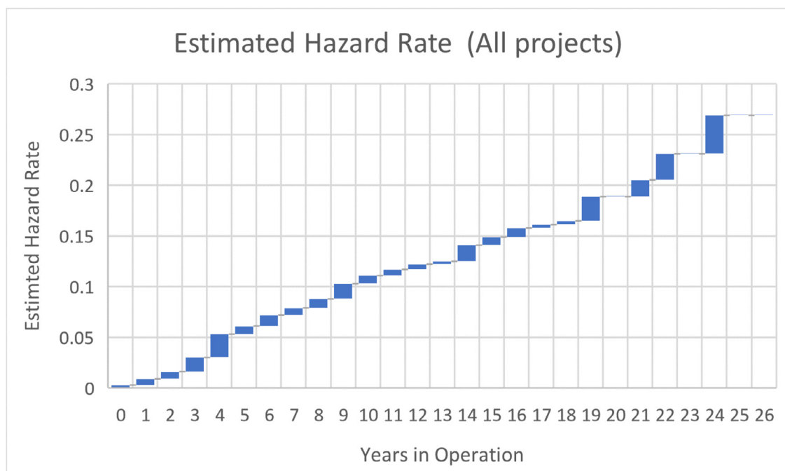
Fig. 3. Estimated year by year hazard rate as reported in Table 4.
