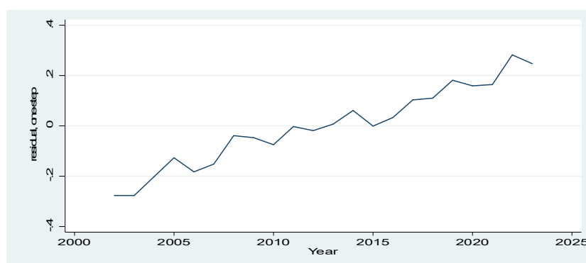
Figure 1. GARCH
