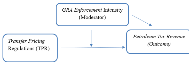
Figure 1. Conceptual Framework
