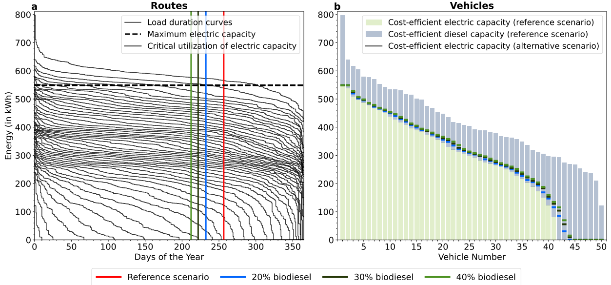
Figure A5. Cost-efficient urban bus fleet. This figure shows (a) the load duration curves of buses in the fleet and (b) the cost-efficient capacity of the electric and diesel drivetrains of the buses across alternative blend levels for biodiesel. The cost-efficient diesel capacity of each vehicle is given by the difference between the upper end of the blue bar and the colored line of a particular scenario.
