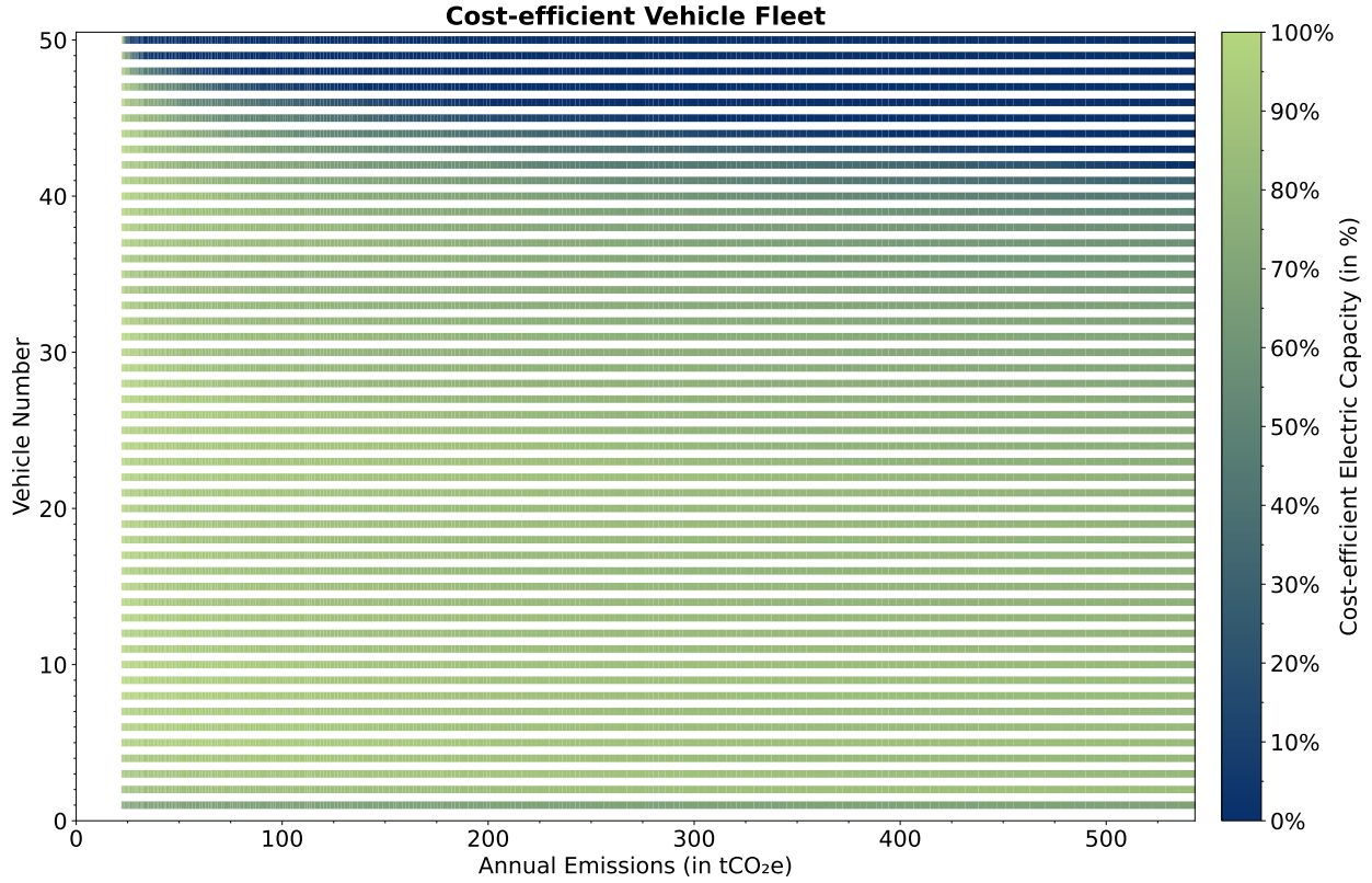
Figure 4. Cost-efficient decarbonization of urban buses. This figure shows the cost-efficient configuration of buses in the fleet corresponding to different emission levels.
