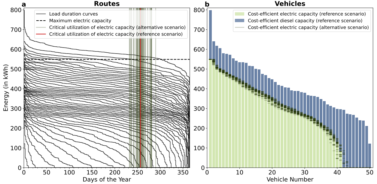
Figure A1. Cost-efficient urban bus fleet. This figure shows (a) the load duration curves of buses in the fleet and (b) the cost-efficient capacity of the electric and diesel drivetrains of the buses, assuming small simultaneous deviations in the costs of vehicles and drivetrains. The cost-efficient diesel capacity of a bus is the difference between the upper end of its blue bar and the dark green lines.
