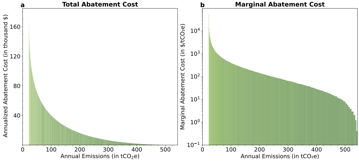
Figure 3. Abatement cost curves for urban buses. This figure shows (a) the annualized total abatement cost and (b) the marginal abatement cost for the urban bus fleet.
