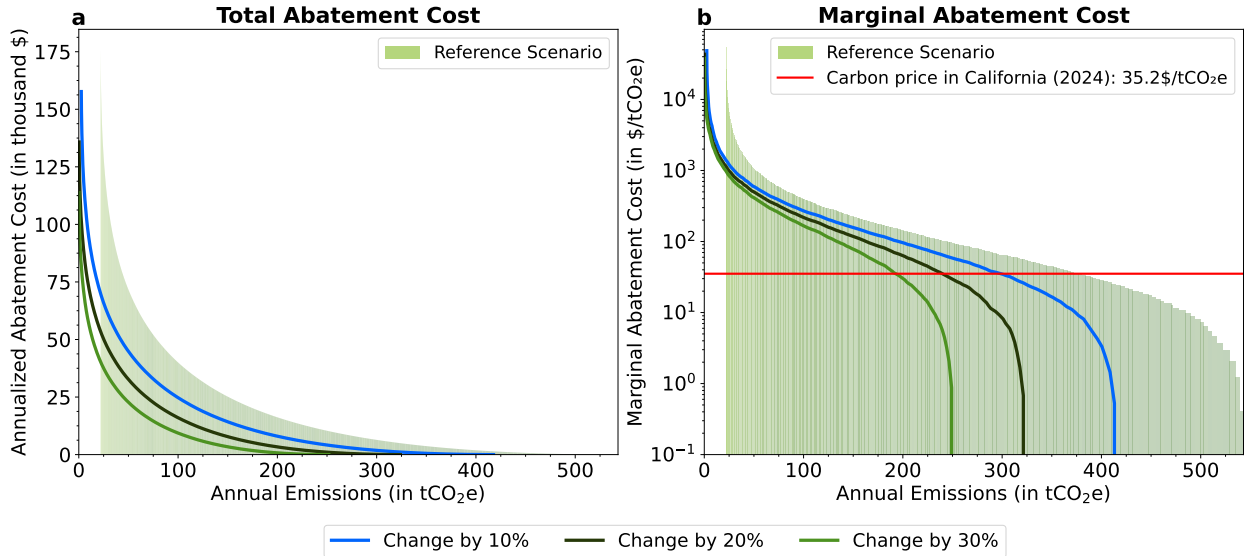
Figure A4. Abatement cost curves for urban buses. This figure shows (a) the annualized total abatement cost and (b) the marginal abatement cost for the urban bus fleet across alternative improvements in battery technology.
