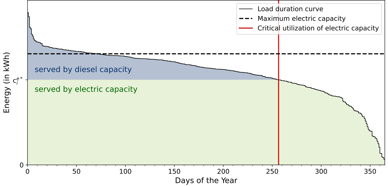
Figure 1. Cost-efficient configuration and deployment of a vehicle. This figure illustrates the load duration curve, critical utilization of the electric capacity, cost-efficient electric capacity, and cost-efficient deployment of vehicle i .
