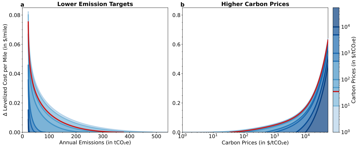
Figure 6. Change in the levelized cost per mile of urban buses. This figure shows (a) the resulting change in the levelized cost per mile, \Delta LCM(E^+|p) , when firms seek to reduce emissions from E^*(p) to some target E^+ and (b) the resulting change in the levelized cost per mile, \Delta LCM(p^+|p) , when the prevailing carbon price increases from p to p^+ .
