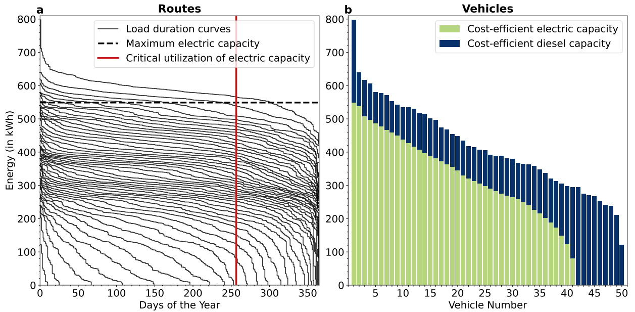
Figure 2. Cost-efficient urban bus fleet. This figure shows (a) the load duration curves of buses in the fleet and (b) the cost-efficient capacity of the electric and diesel drivetrains of the buses.
