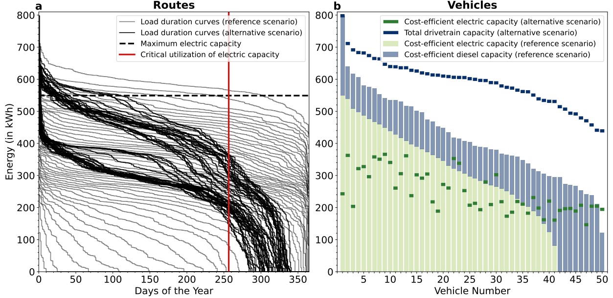
Figure A7. Cost-efficient urban bus fleet. This figure shows (a) the load duration curves of buses in the fleet and (b) the cost-efficient capacity of the electric and diesel drivetrains of the buses, assuming no reassignment of vehicles to routes. The cost-efficient diesel capacity of each vehicle is given by the difference between the dark blue line and the dark green line.
