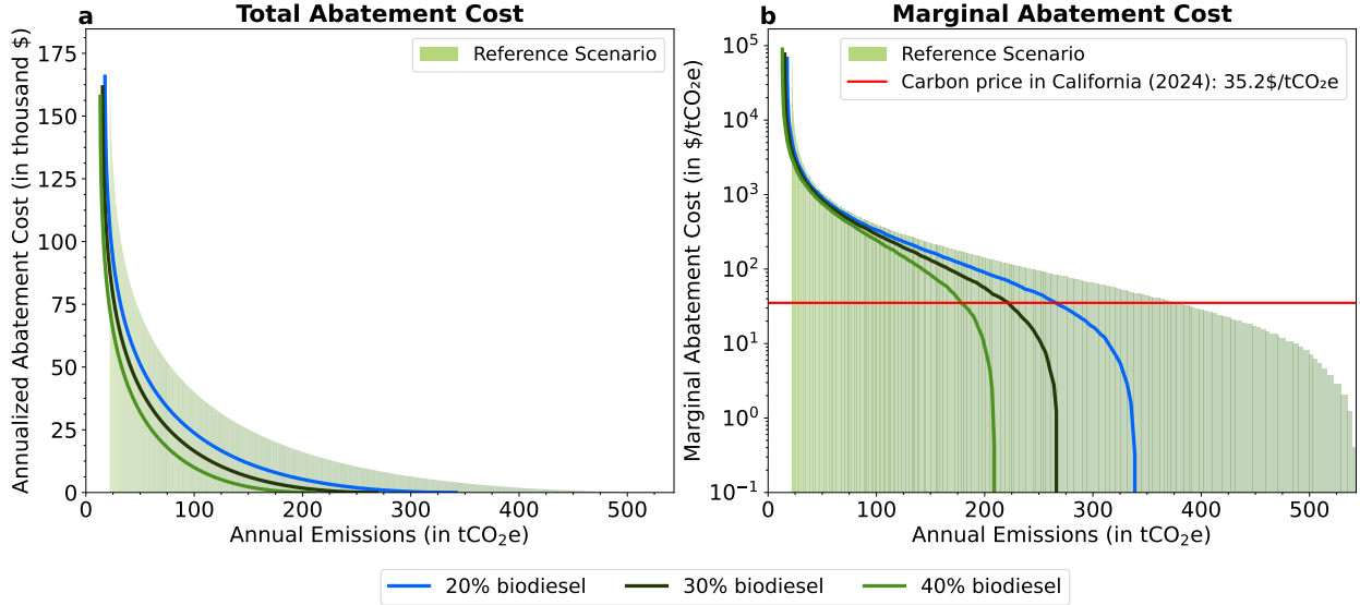
Figure A6. Abatement cost curves for urban buses. This figure shows (a) the annualized total abatement cost and (b) the marginal abatement cost for the urban bus fleet across alternative blend levels for biodiesel.
