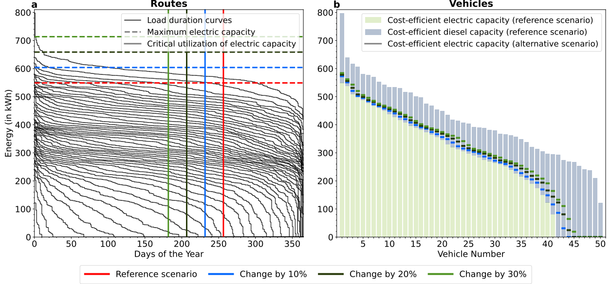
Figure A3. Cost-efficient urban bus fleet. This figure shows (a) the load duration curves of buses in the fleet and (b) the cost-efficient capacity of the electric and diesel drivetrains of the buses across alternative improvements in battery technology. The cost-efficient diesel capacity of each vehicle is given by the difference between the upper end of the blue bar and the colored line of a particular scenario.
