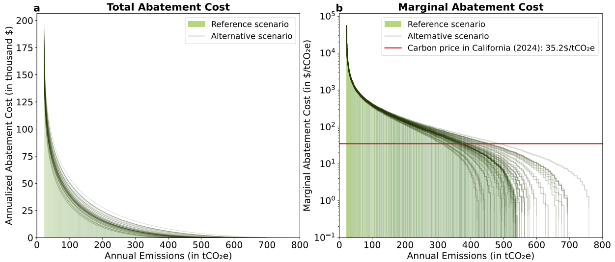
Figure A2. Abatement cost curves for urban buses. This figure shows (a) the annualized total abatement cost and (b) the marginal abatement cost for the urban bus fleet, assuming small simultaneous deviations in the costs of vehicles and drivetrains.
