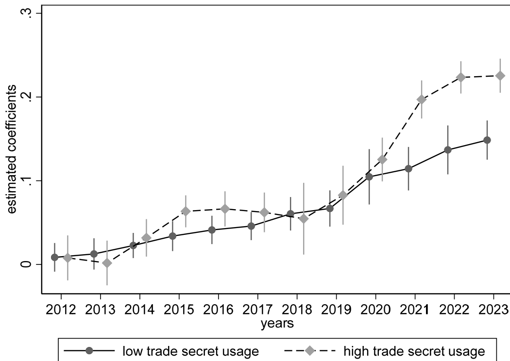
Figure 1: Trends in Trade Secret Declaration in Industries with High and Low Trade Secret Reliance
