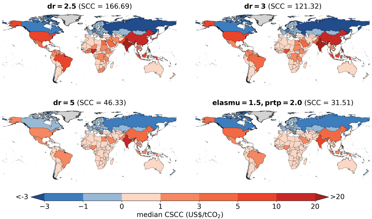
Figure B.5: Median country-level social cost of carbon (CSCC) under alternative discounting assumptions.
