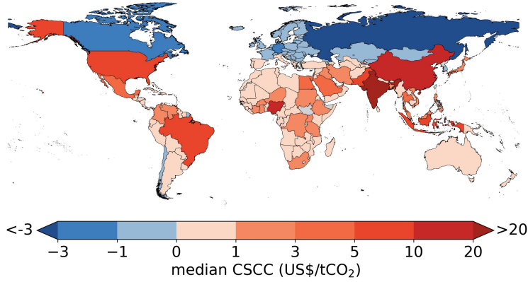
Figure 2: Median country-level social cost of carbon (CSCC).
