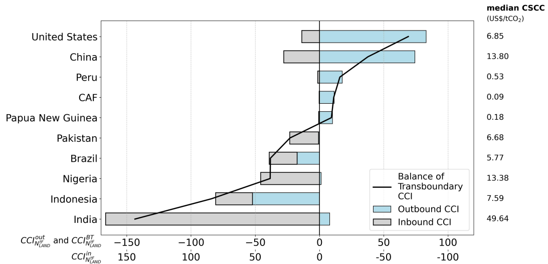
Figure 4: Top and bottom five countries by balance of transboundary CCI from the net land carbon flux N_{LAND}^{IF} .
