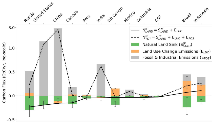
Figure B.2: Carbon flux breakdown for major land sinks (2013–2022).
