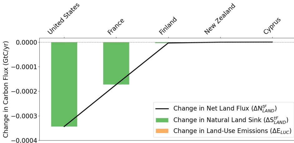
Figure B.4: Effect of attributing overseas territories on national carbon flux estimates.
