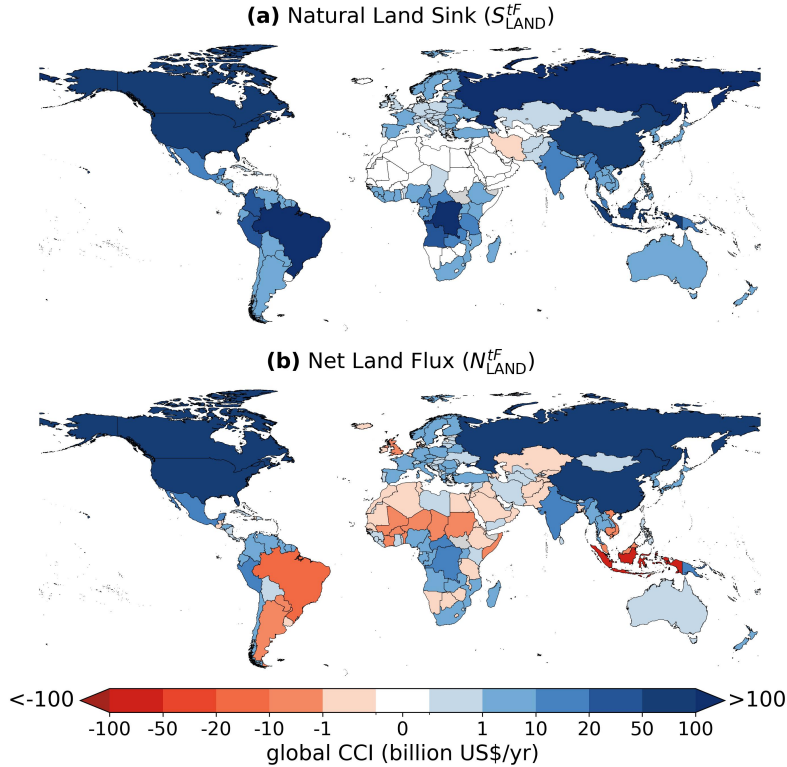
Figure 3: Country-level global carbon flux contributions to comprehensive investment (CCI).
