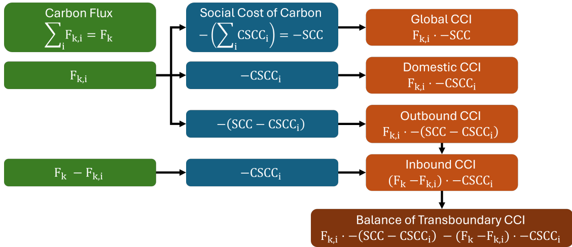
Figure B.1: Schematic overview of carbon flux contributions to comprehensive investment (CCI).
