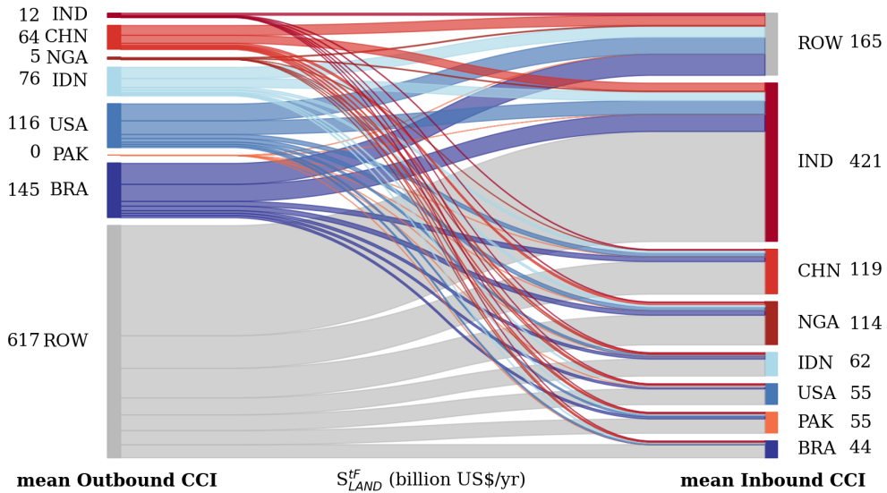
Figure 5: Outbound and inbound CCI from the natural land sink ( S_{LAND}^{IF} ) for the seven countries with the highest CSCC.
