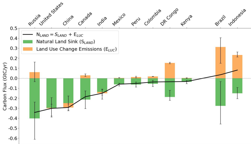
Figure B.3: Carbon flux breakdown for major land sinks (2013–2022).
