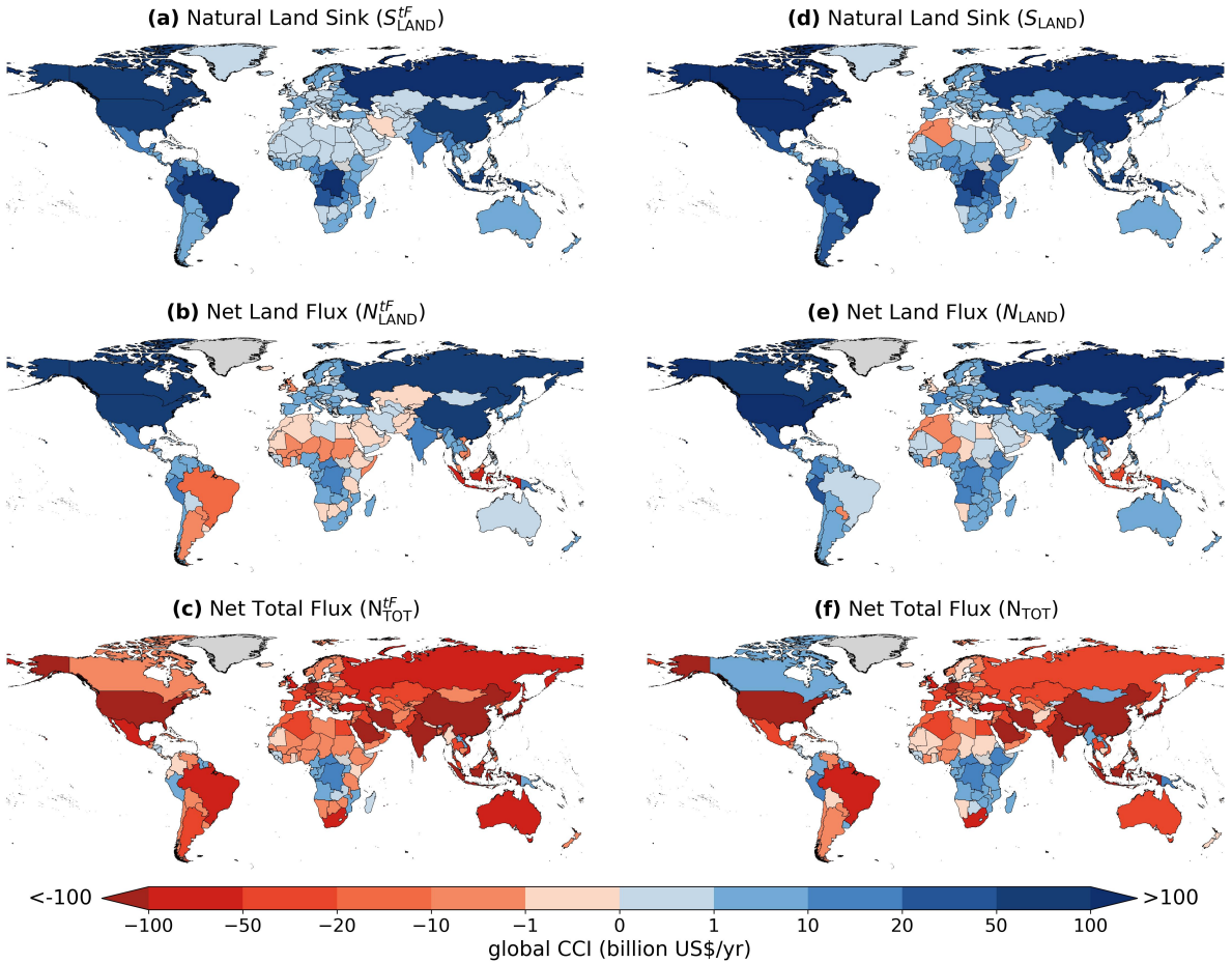
Figure B.6: Global carbon flux contributions to comprehensive investment based on present-day forest area and pre-industrial land covers.
