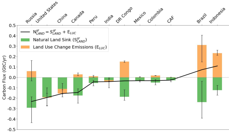
Figure 1: Carbon flux breakdown for major land sinks (2013–2022).
