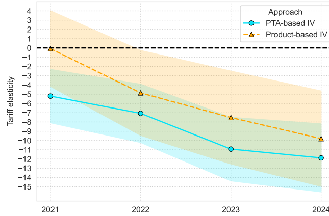
Figure 4: Dynamics of the tariff elasticity, IV regressions
