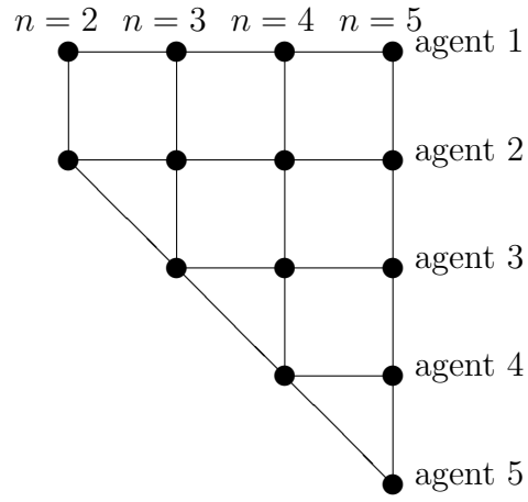
Figure 3: Comparisons top-down
