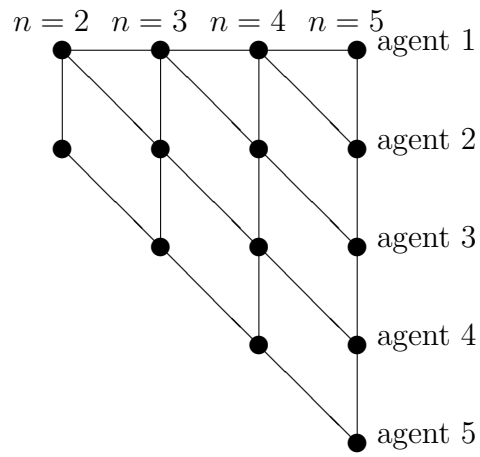
Figure 4: Comparisons bottom-up
