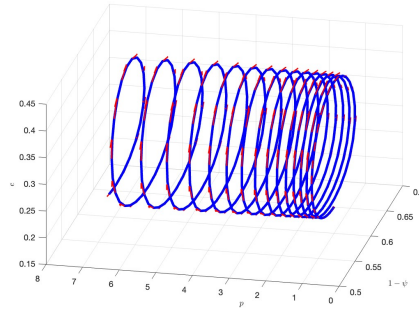
(c) Phase portrait: profit-price spiral induced by \varepsilon = 0.99
