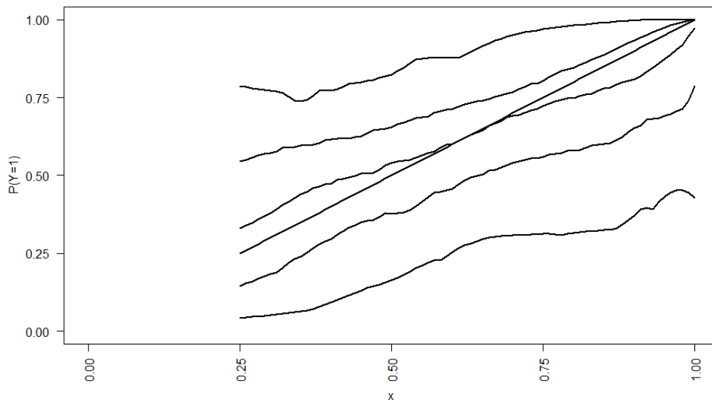
Figure 5. Distribution of the probability of giving a correct answer among the students shown by the 5:th, 25:th, 50:th, 75:th and 95:th percentile for various confidence levels. The straight line represents perfect self-awareness, P(Y = 1) = x .
