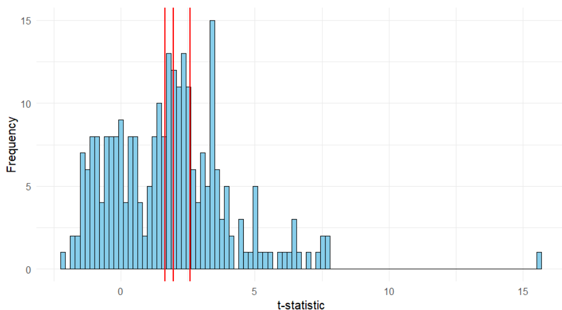
Figure 4: T-statistic distribution
