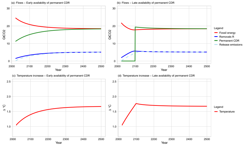
FIGURE 4. Numerical simulations for early (left panels) and late (right panels) availability of permanent CDR. Upper panels show flows over time, bottom panels show the temperature.
