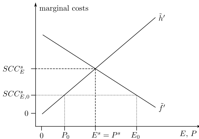
FIGURE 3. In an optimal steady state, the atmospheric carbon stock adjusts so that the SCC_E are at the unique level at which permanent removals exactly offset residual emissions.
