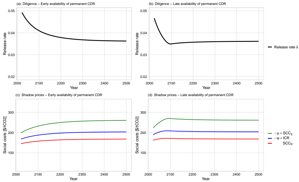
FIGURE D.1. Time paths of optimal diligence and the shadow prices -\mu and -\psi for the model runs in Figure 4.
