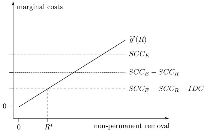
FIGURE 2. Optimality condition for non-permanent removals
