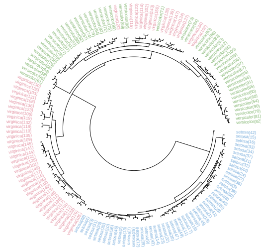
(c) Average-Linkage
