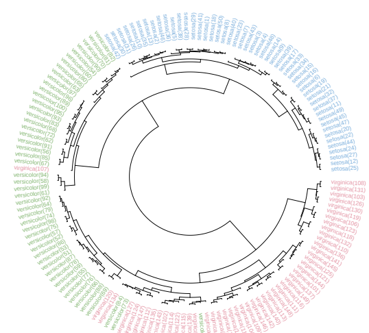
(b) Complete-Linkage
