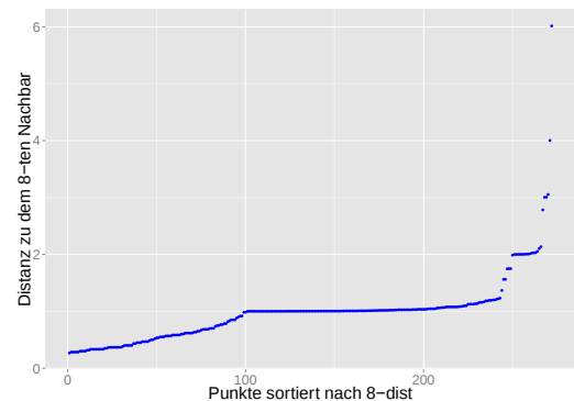
(c) 8-dist Plot
