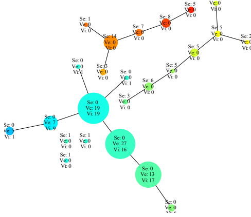
(a) Mapper(f^{-1}(\mathcal{V}(15, 0.25), \mathcal{C}))
