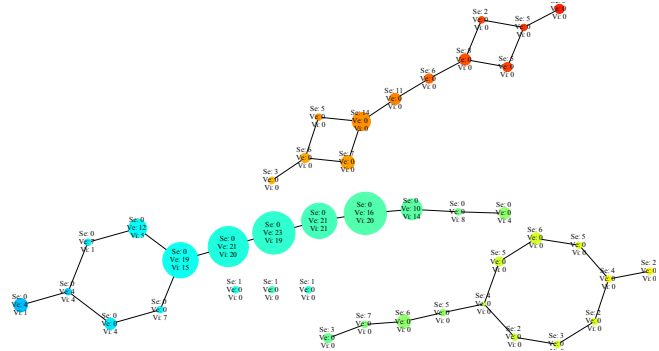
(c) \text{Mapper}(f^{-1}(\mathcal{V}(30, 0.95), \mathcal{C}))
