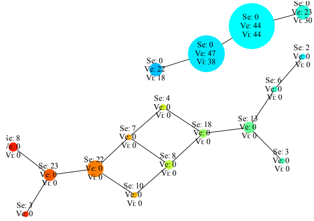
(a) \text{Mapper}(f^{-1}(\mathcal{V}(10, 0.95), \mathcal{C}))
