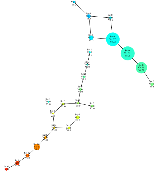
(b) Mapper(f^{-1}(\mathcal{V}(15, 0.45), \mathcal{C}))
