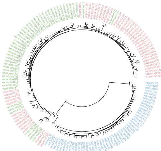
(a) Single-Linkage
