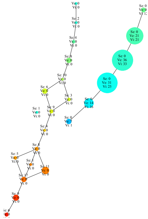
(c) Mapper(f^{-1}(\mathcal{V}(15, 0.65), \mathcal{C}))
