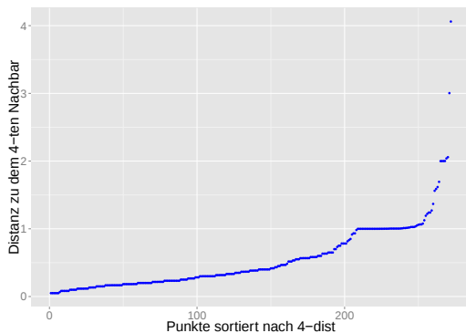
(b) 4-dist Plot
