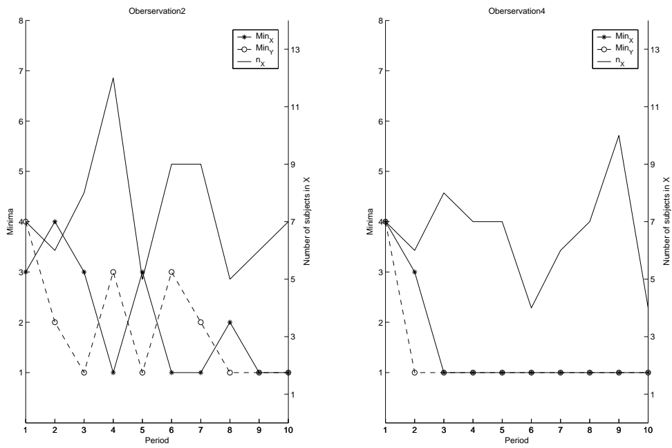
Figure 8: Coordination patterns.
