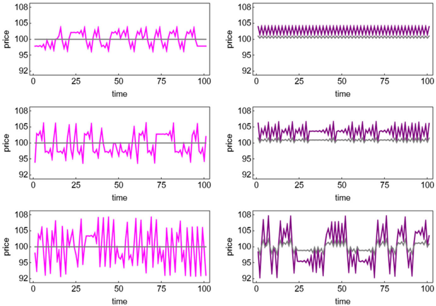
Fig. 3 The left panels show the evolution of the price (pink) and the perceived fundamental (gray) for d = 0 . The right panels show the evolution of the price (purple) and the perceived fundamental (gray) for d = 0.25 . The top, middle, and bottom panels are based on our parameter setting, except that b = 6 , b = 10 , and b = 15 , respectively (color figure online)
