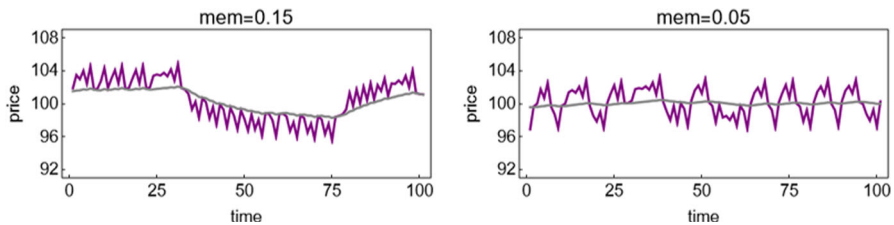
Fig. 8 The left panel shows the evolution of the price (purple) and the perceived fundamental value (gray) for d = 0.6 and mem = 0.15 . The right panel shows the evolution of the price (purple) and the perceived fundamental value (gray) for d = 0.6 and mem = 0.05 (color figure online)
