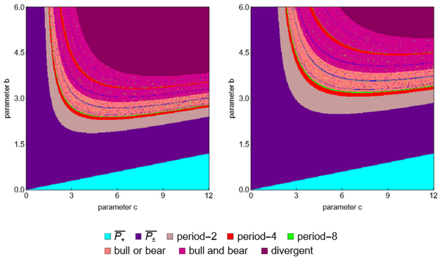
Fig. 1 The left (right) panel presents a two-dimensional bifurcation diagram in the parameter plane (c, b) for d = 0 ( d = 0.25 )
