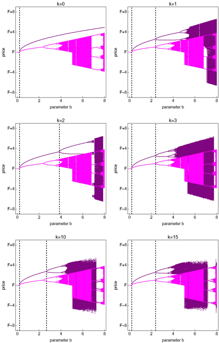
Fig. 5 The panels show the bifurcation diagrams in which the price is depicted versus parameter b for d = 0 (magenta) and d = 0.6 (purple) for different values of k = 0, 1, 2, 3, 10, 15 (color figure online)
