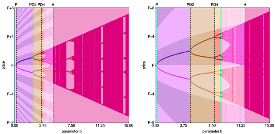
Fig. 2 The left (right) panel shows the bifurcation diagram in which the price is depicted versus parameter b for d = 0 ( d = 0.25 )
