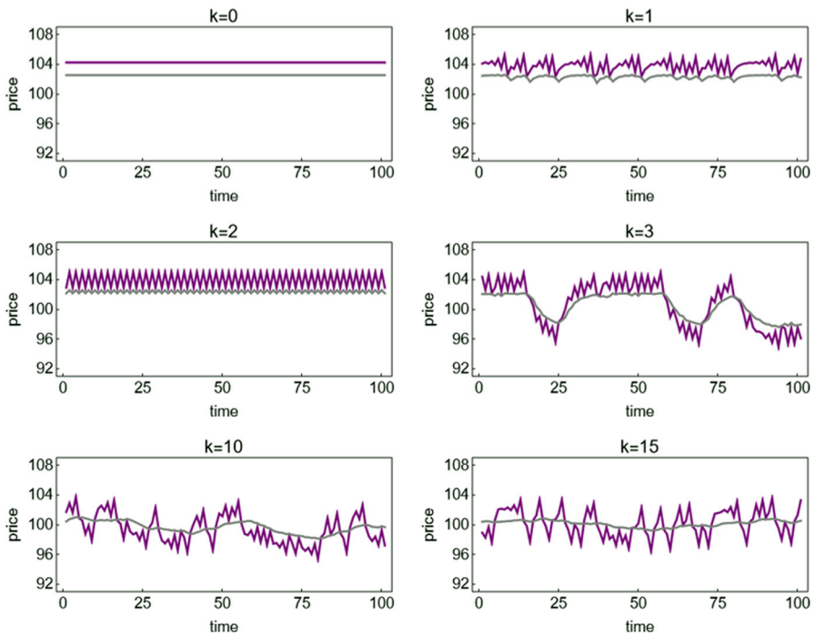
Fig. 6 The panels show the evolution of the price (purple) and the perceived fundamental value (gray) for d = 0.6 and different values of k = 0, 1, 2, 3, 10, 15 (color figure online)
