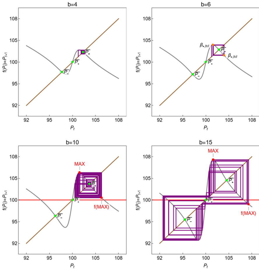
Fig. 4 The panels present the evolution of the price in the phase diagram for d = 0.25 and different values of b = 4, 6, 10, 15 . The green dots indicate the steady states. The orange dots indicate the periodic point of the period-two cycle
