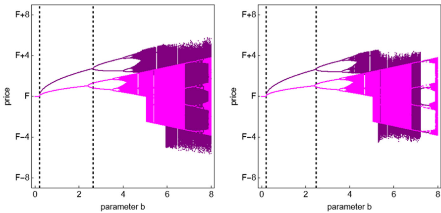
Fig. 7 The left panel shows the bifurcation diagram plotting price versus parameter b for d = 0 (magenta) and d = 0.6 (purple) for mem = 0.15 . The right panel shows the bifurcation diagram plotting price versus parameter b for d = 0 (magenta) and d = 0.6 (purple) for mem = 0.05 (color figure online)
