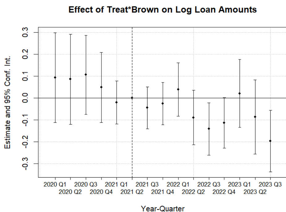
Figure 2: Time-varying coefficients
