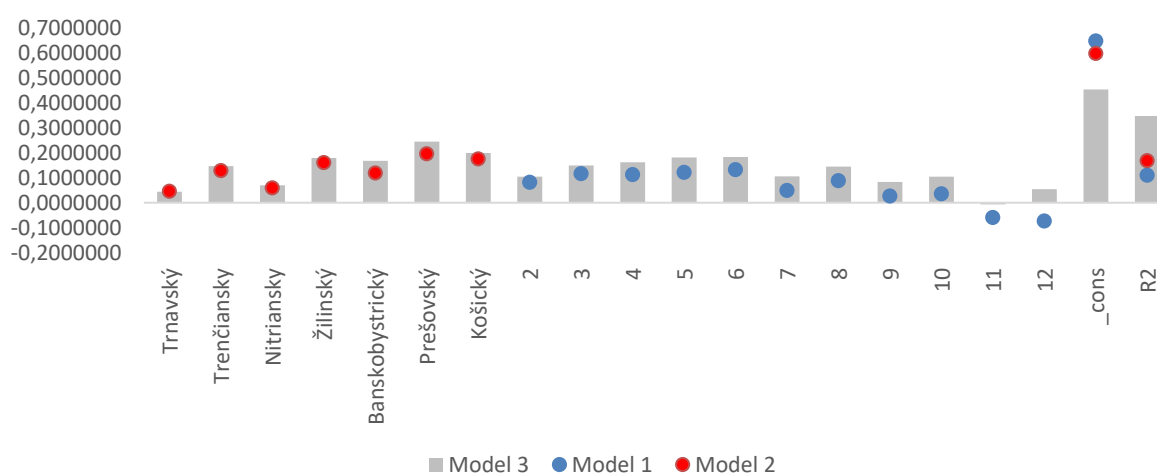
Fig. 6. Comparison of model coefficients.
