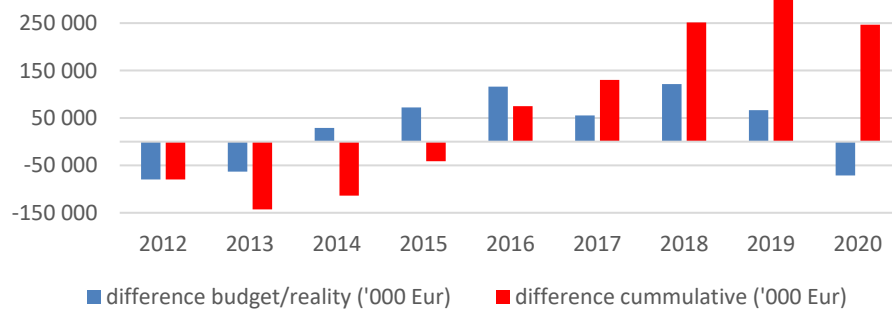
Fig. 5. Evolution of the difference between the budgeted and the actual PIT yield.
