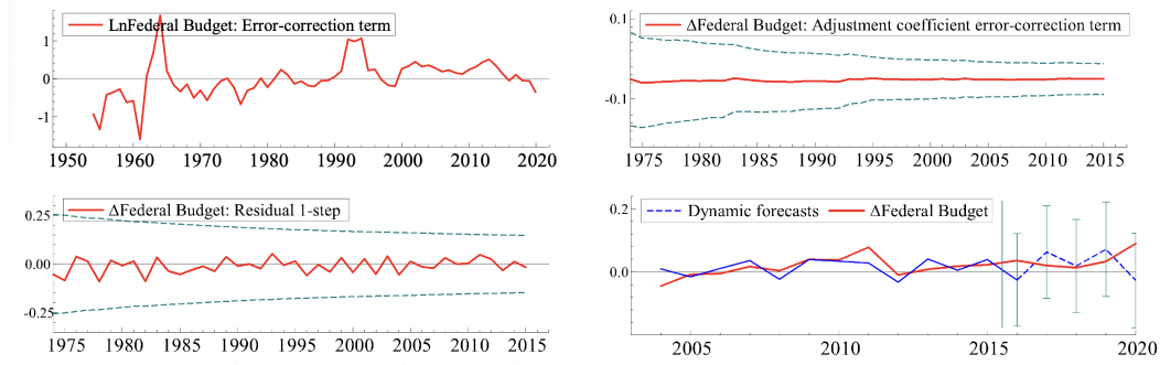
Figure 4: Federal Budget: Error-correction term, recursive estimation of adjustment coefficient on error-correction term, 1-step residual and 1-step out-of-sample dynamic forecasts.
