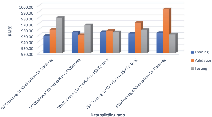
Figure 5. Performance of ANN-1 variations in terms of RMSEs: different data segmentation ratios
