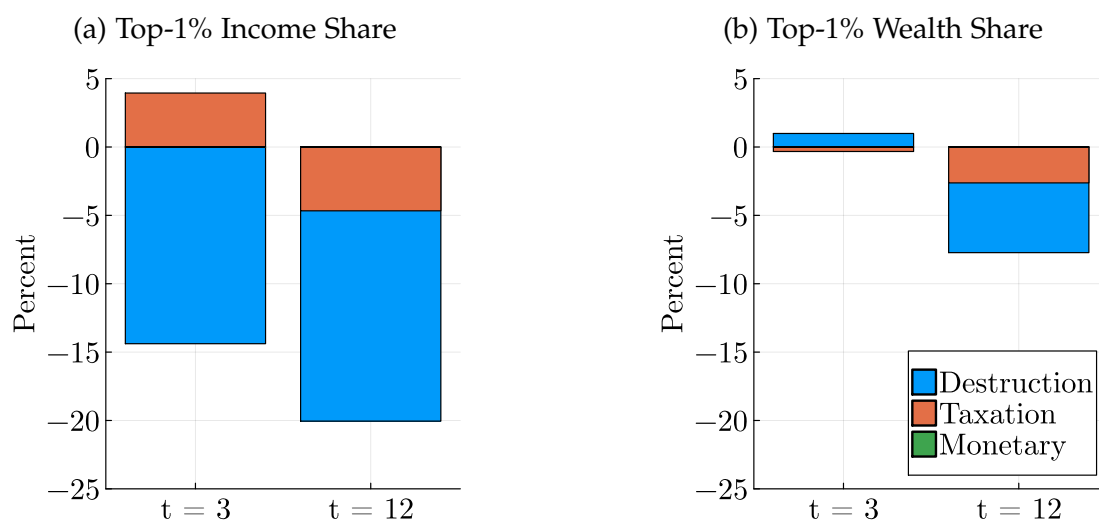
Figure 8: Shock decomposition
