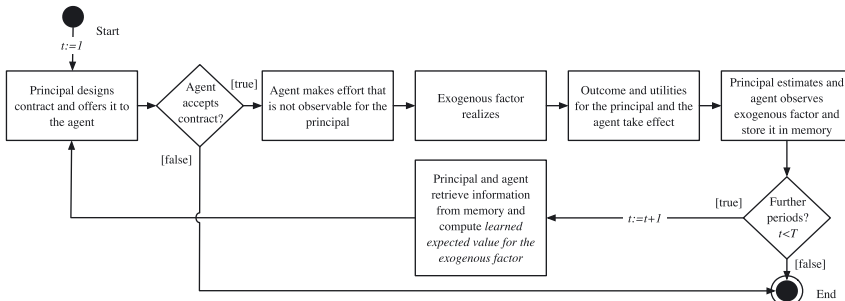
Figure 2: Sequence of events in the agent-based model.
