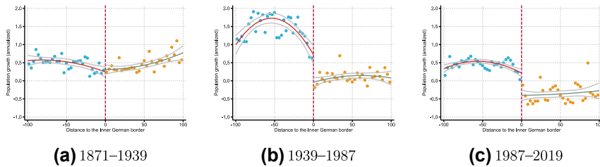
Figure 3: Population growth at the Inner German border. The figure plots annualized population growth rates in German municipalities between (a) 1871 and 1939, (b) 1939 and 1987, and (c) 1987 and 2019 against their distance to the 1945–1990 Inner German border (maximum distance: 100 km). Negative values refer to West Germany, positive values to East Germany. The corresponding local-linear regression discontinuity estimates (Calonico et al. 2017) are (a) 0.0468 ( p = 0.621 ), (b) -0.735 ( p = 0.000 ), and (c) -0.401 ( p = 0.000 ). Data: GPOP Version 1.0.
