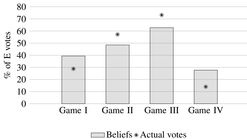
Figure F.3. Beliefs about % of E votes and actual % of E votes with restricted sample
