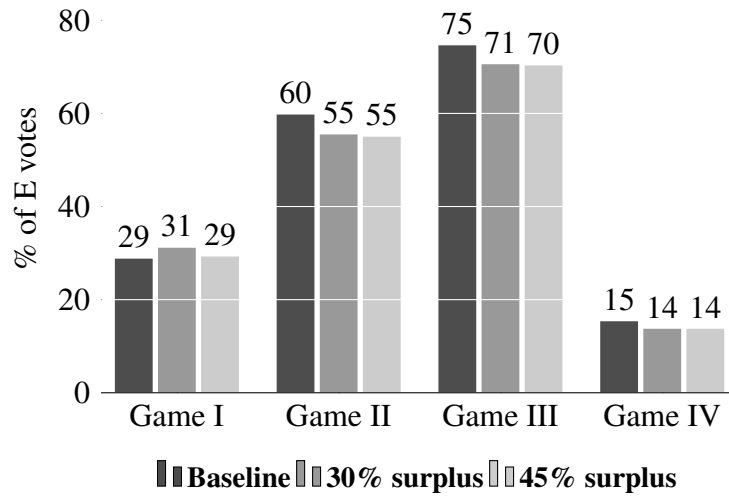
Figure F.2. % of E votes with Baseline (a1), 30% surplus gain (a4), and 45% surplus gain (a5) with restricted sample
