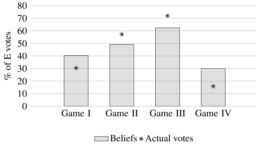
Figure 5. Beliefs about percentages of E votes and actual percentages of E votes
