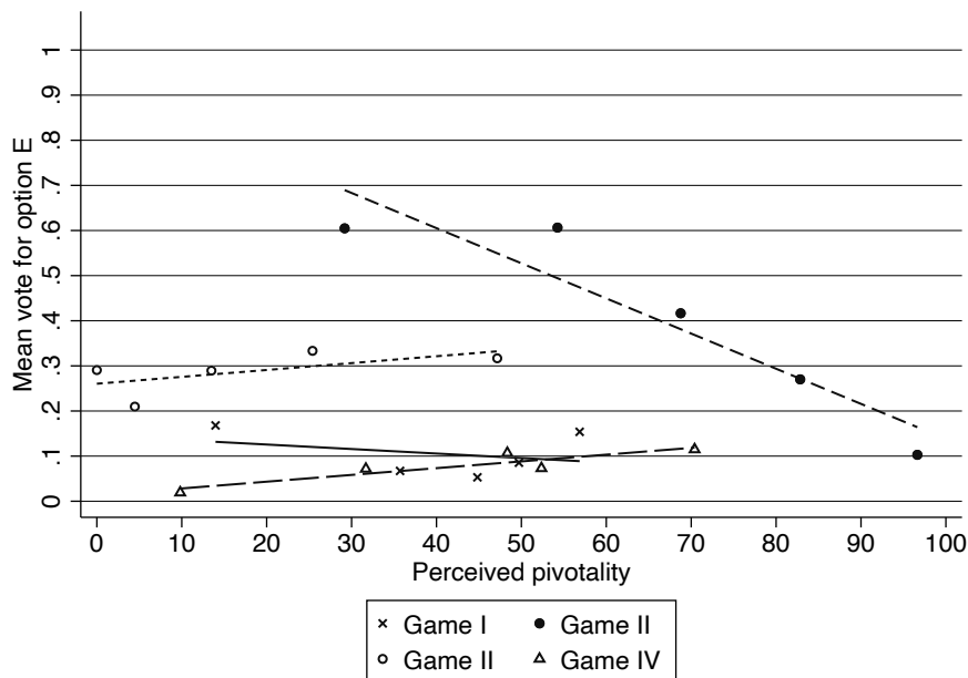
Figure F.5. Cheap fairman talk per game with restricted sample
