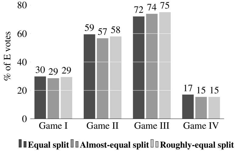
Figure 3. Percentage of E votes across equal split (a1), almost-equal split (a2), and roughly-equal split (a3)
