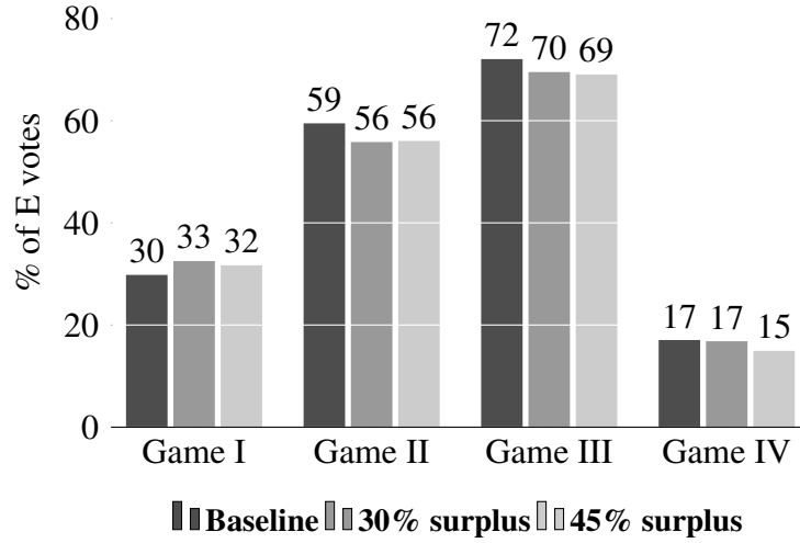
Figure 4. Percentages of E votes with baseline (a1), 30% surplus gain (a4), and 45% surplus gain (a5)
