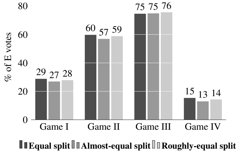
Figure F.1. % of E votes across equal split (a1), almost-equal split (a2), and roughly-equal split (a3) with restricted sample
