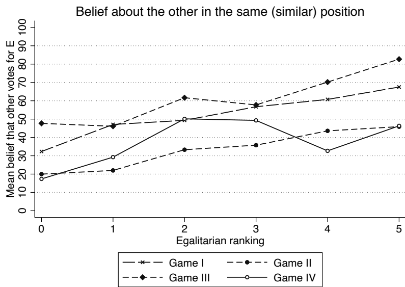
Figure F.4. False-consensus bias per game with restricted sample
