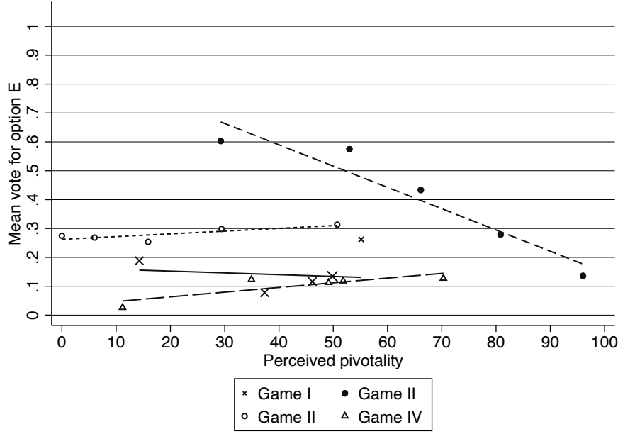
Figure 8. Cheap fairman talk per game
