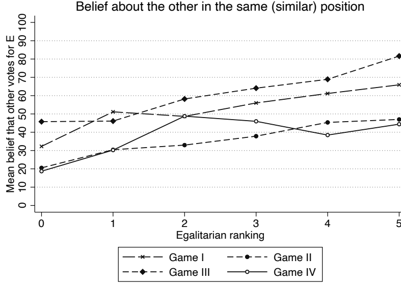
Figure 7. False-consensus bias per game
