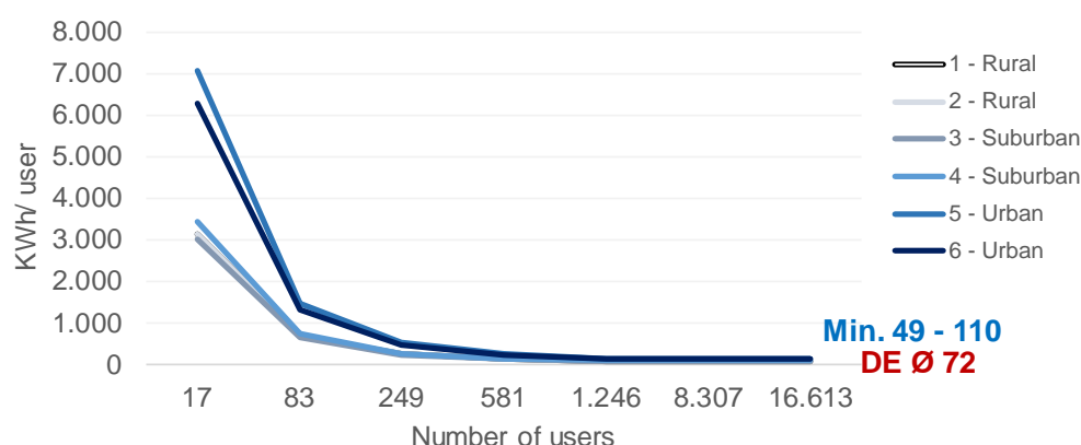
Figure 5: Mobile access network – Energy curves by number of users and population densities
