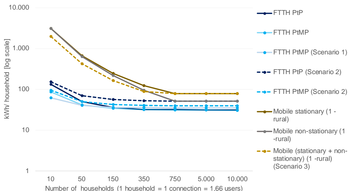
Figure 7: Comparison of energy curves between FTTH and mobile access networks under different scenarios
