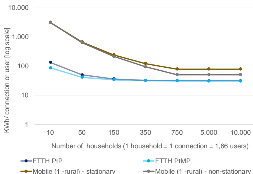
Figure 6: Fibre vs. mobile access networks – energy consumption by population size
