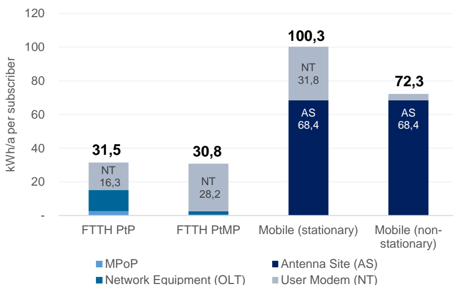
Figure 3: Contribution of network elements to average energy consumption in Germany by technology (kWh per connection or mobile user per year) 52
