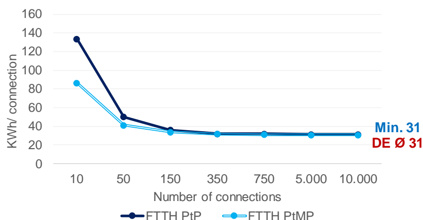
Figure 4: Fibre access network – Energy curves by number of connections
