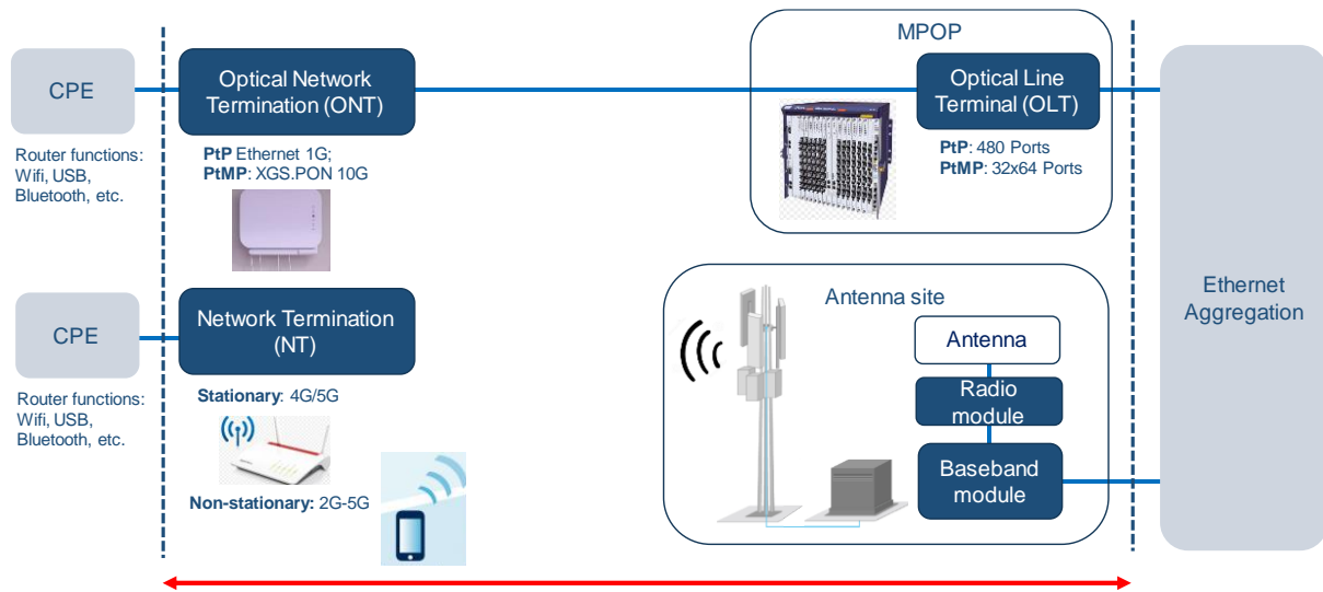
Figure 1: Graphical representation of system boundaries of fibre access networks (FTTH) and mobile access networks
