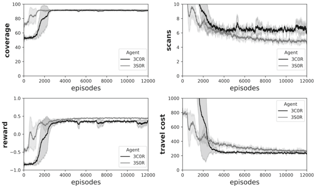
Fig. 6 Trajectory of evaluated performance indicators and reward of two exemplary agent configurations over the course of learning. Top left: Trajectory of the object surface coverage. Top right: Trajectory of
