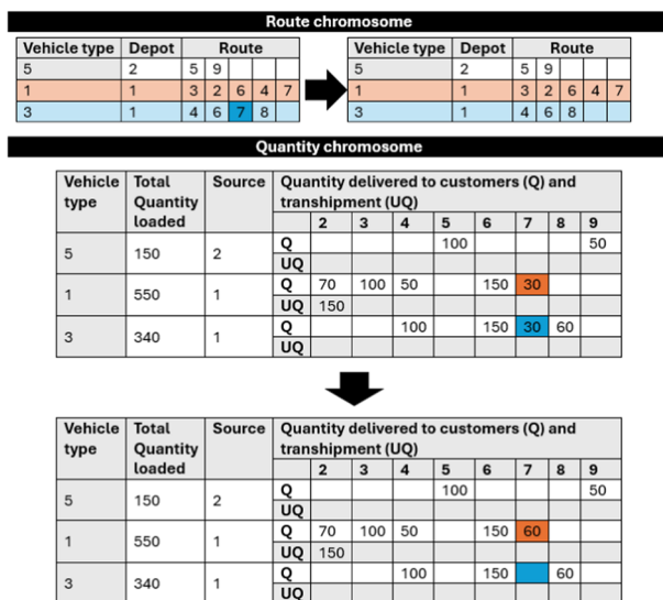
Fig. 19 Illustration of Operator 15
