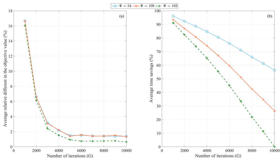
Fig. 6 Average relative difference in the objective value and time savings with respect to the best heuristic solution found as a function of the number of iterations for different numbers of individuals
