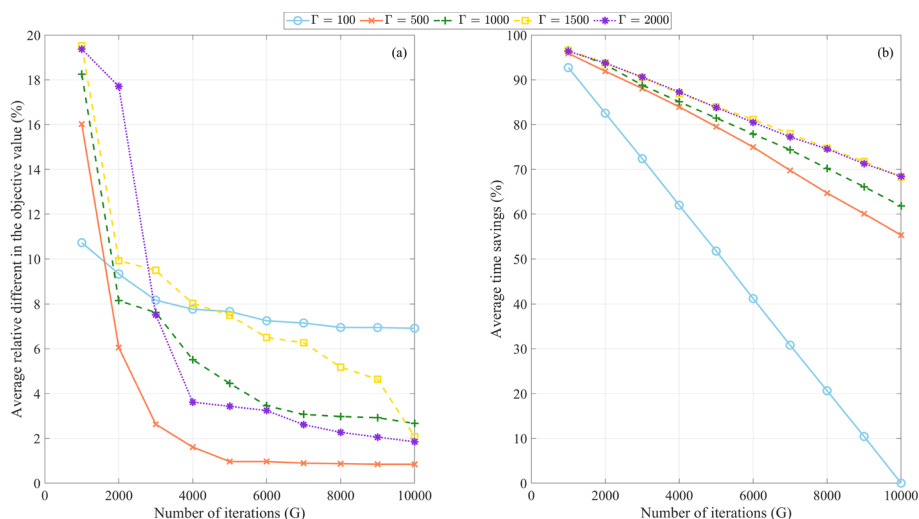
Fig. 5 Average relative difference in the objective value and time savings with respect to the best heuristic solution found as a function of the number of iterations for different numbers of iterations without improvement
