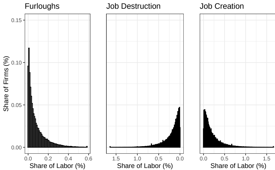
Figure 2: Histograms of reallocation and furloughs
