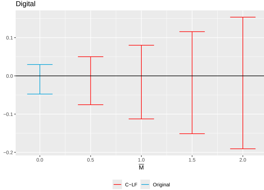
Figure 13: Sensitivity analysis of parallel trends assumption for digital volume
