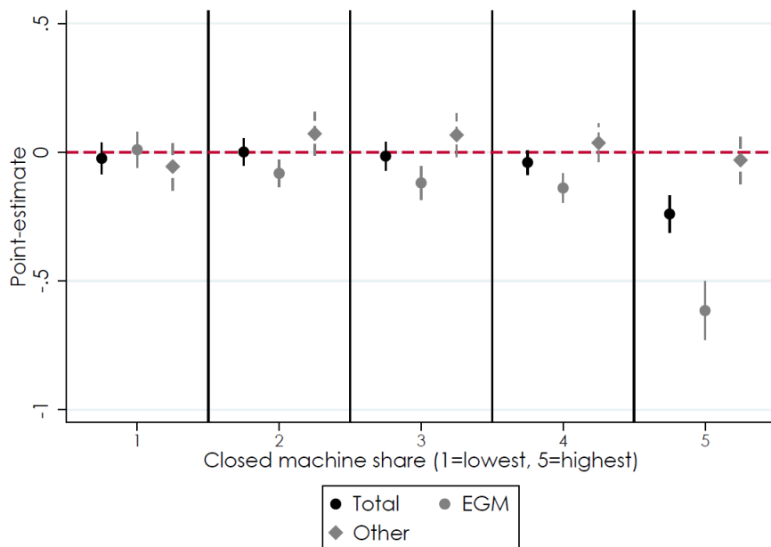
Figure 18: Heterogeneous response: importance of closed outlets
