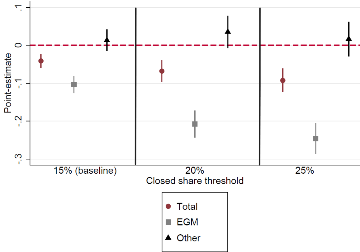
Figure 17: Sensitivity of results to closed share
