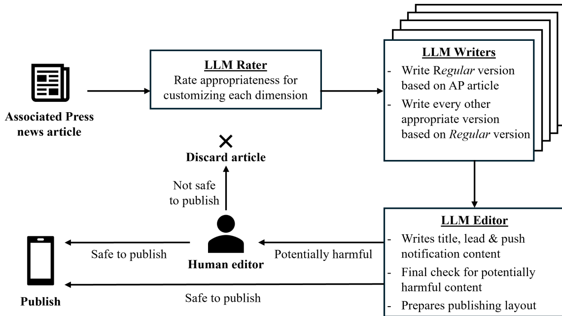
Figure 2: Multi-Agent AI System for Rewrites
