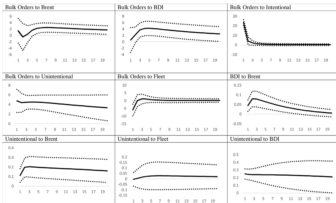
Fig. 3. Impulse responses.
