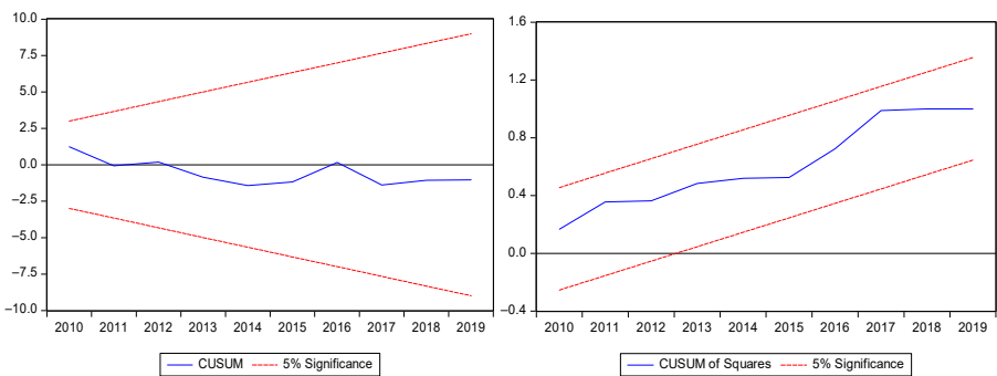
Figure 4. Cusum and cusum of squares
