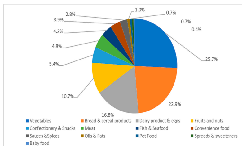
Figure 1. Quantity of food manufactured in the KSA (in thousand tons), distributed by type in 2022.
