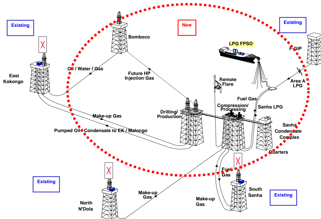
Figure 6.4 Sanha Condensate Project, Angola
