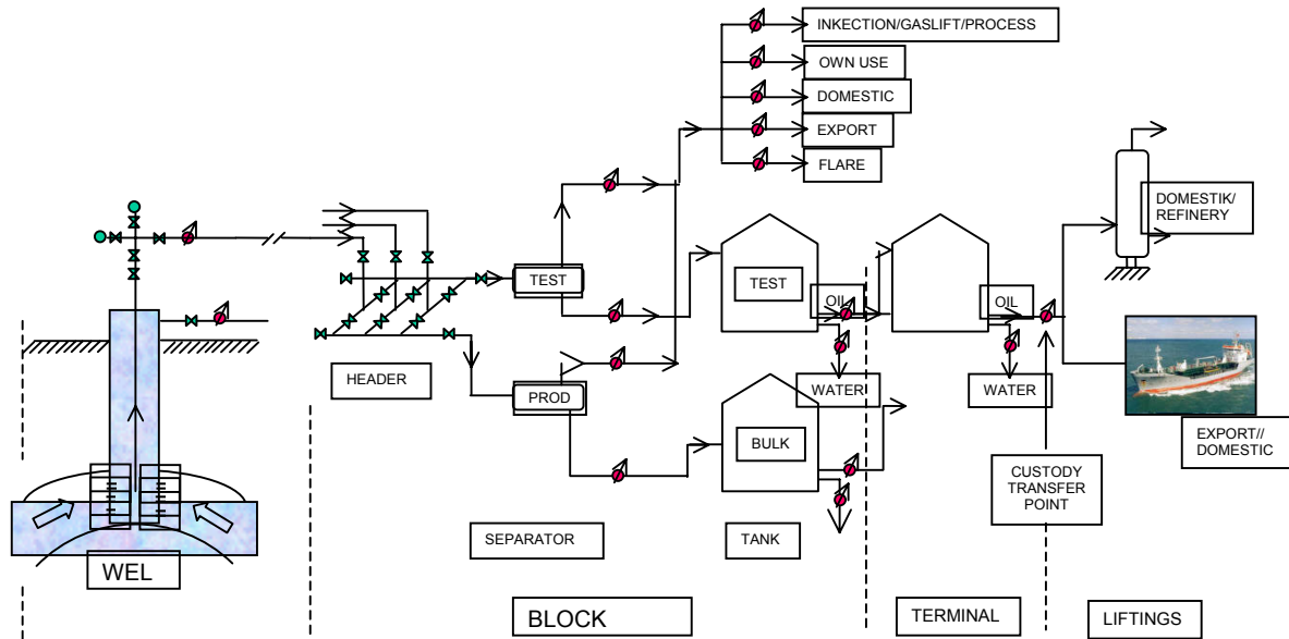
Figure 2.6 Oil and Gas Flow Diagram
