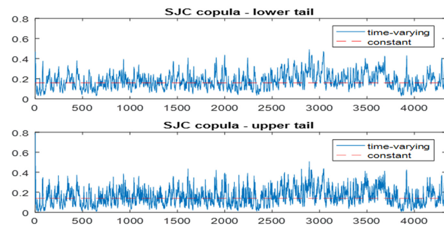
Figure 8. Dependence path of the time-varying SJC: pair oil-telecommunication.
