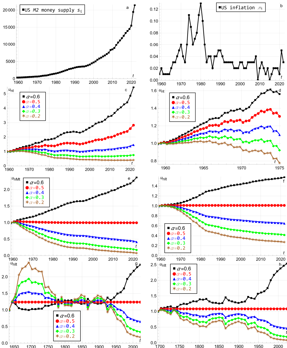
Figure 1. Panel (a): US M2 money supply s_i 1959–2021 in USD billion. Panel (b): US inflation \pi_i 1959–2021. Panels (c–h): The player's utility u_{nt} , u_{nMt} , u_{nIt} as a function of time t for the Cobb–Douglas elasticities \alpha = 0.6, 0.5, 0.4, 0.3, 0.2 . Panel (c): Equation (1) 1959–2021. Panel (d): Equation (1) 1959–1975. Panel (e): Equation (2) 1959–2021 based on money printing empirics. Panel (f): Equation (3) 1959–2021 based on inflation empirics. Panel (g): Equation (3) 1635–2021 based on inflation empirics. Panel (h): Equation (3) 1695–2021 based on inflation empirics.
