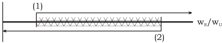
Figure 1: Graphical illustration of proposition 2.1
