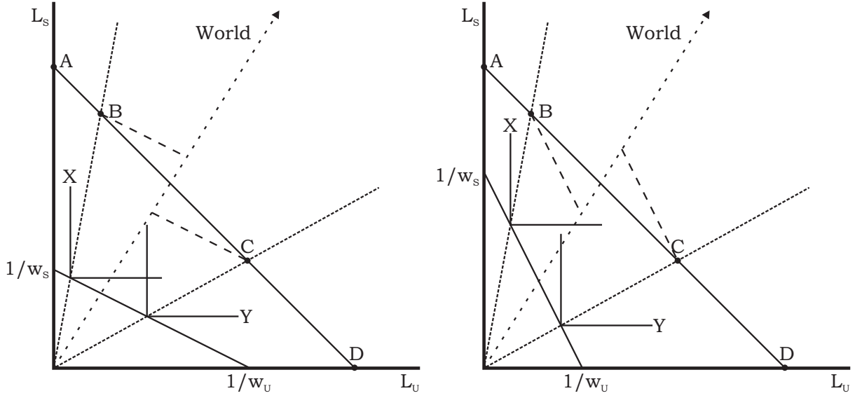
Figure 3: Lerner-Diagram
