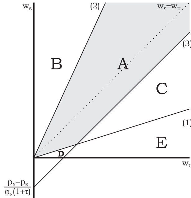
Figure 2: Graphical illustration of conditions (1), (2), (3) and proposition 2.2
