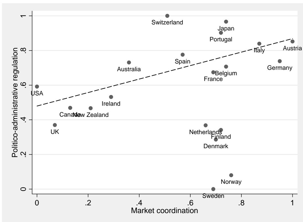
Figure 2: Politico-administrative regulation and market co-ordination (Principal component analysis)
