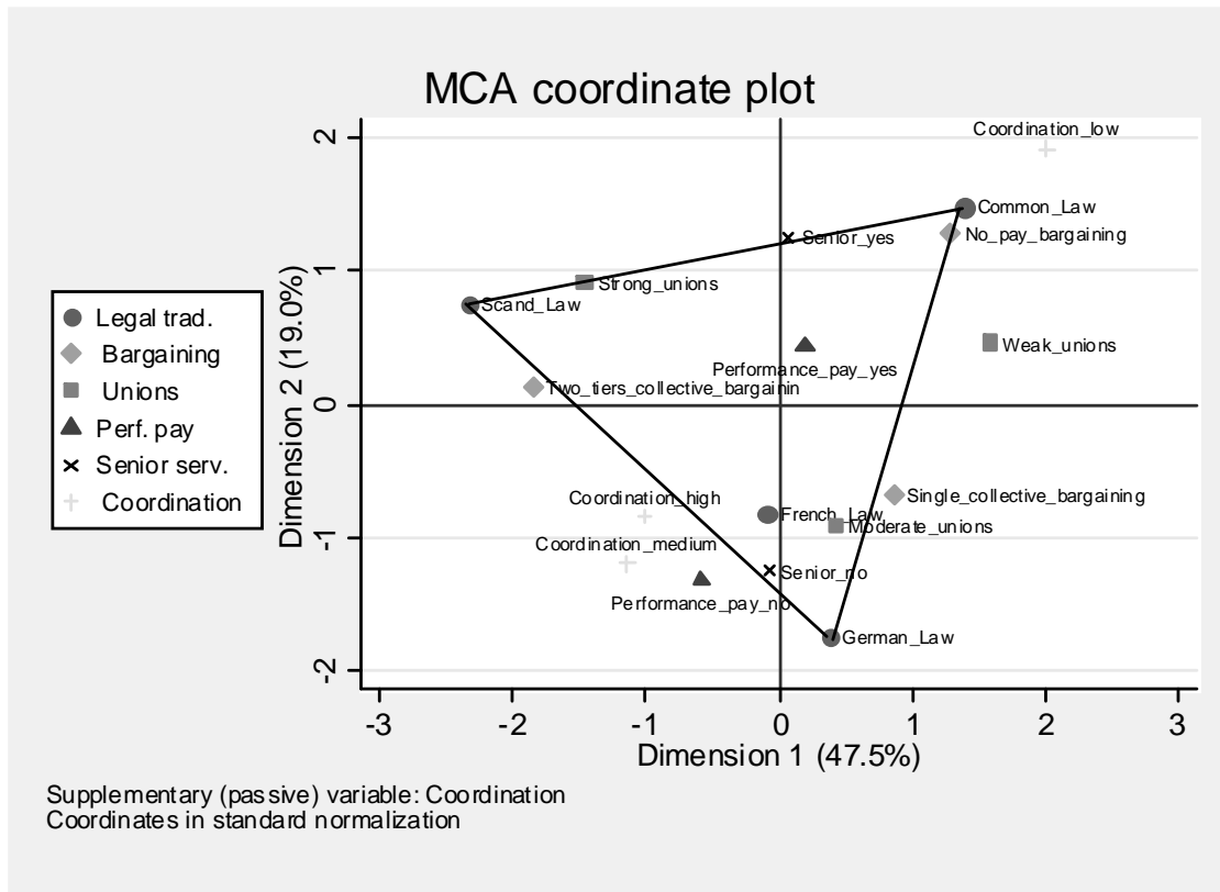
Figure 1: Public employment regulation and market coordination (Multiple correspondence analysis)
