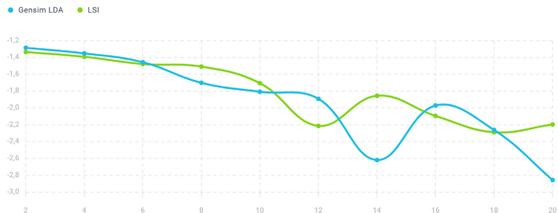
FIG. 2. Coherence scores.
