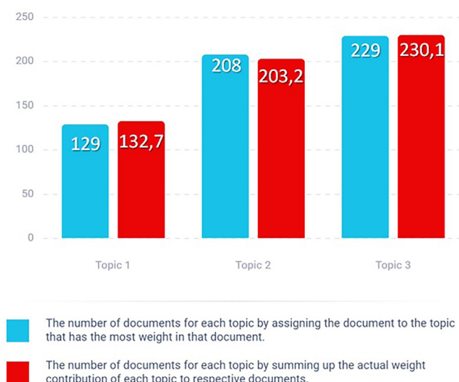
FIG. 4. Topic-documents distribution.
